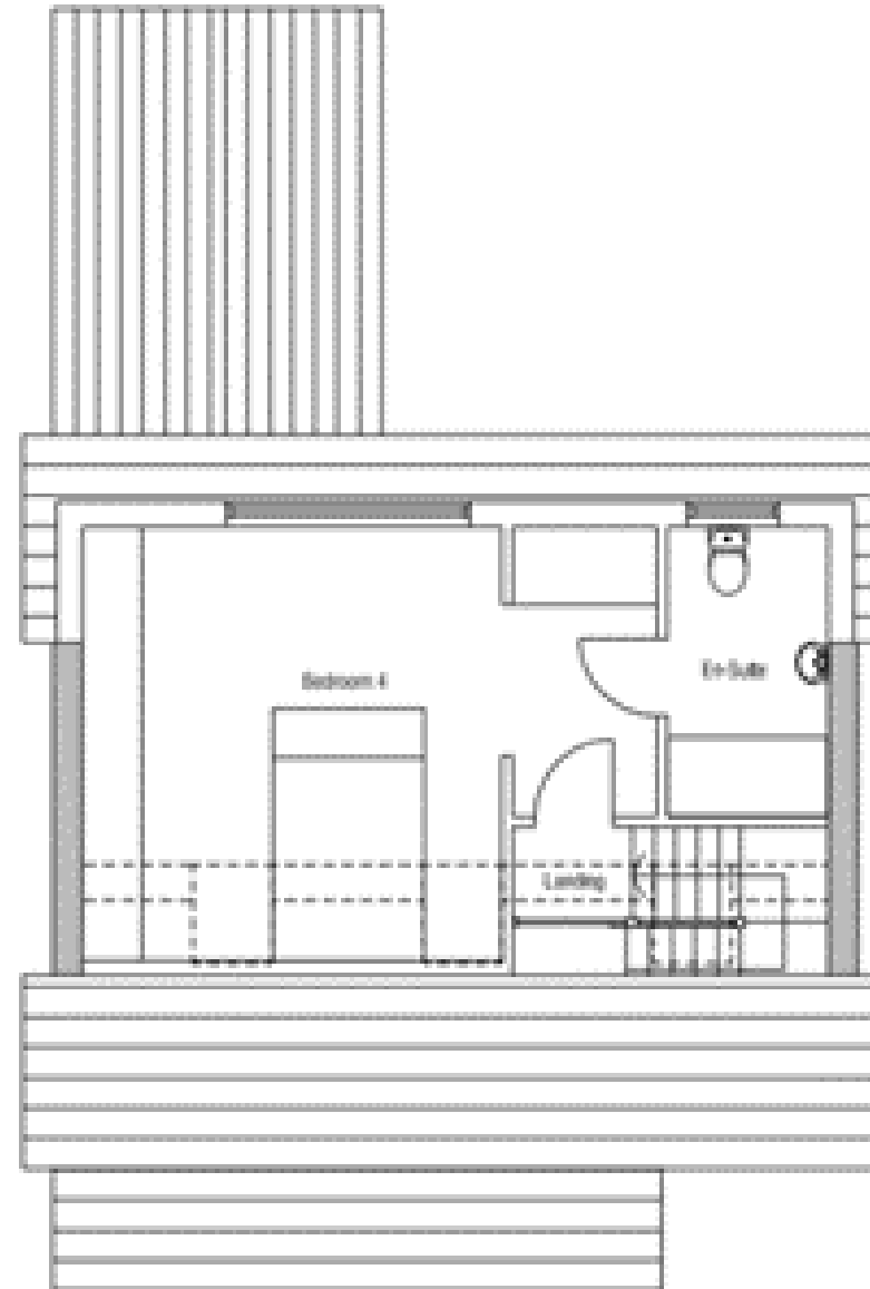
PROPOSED ENCORE FLOOR 1/20
