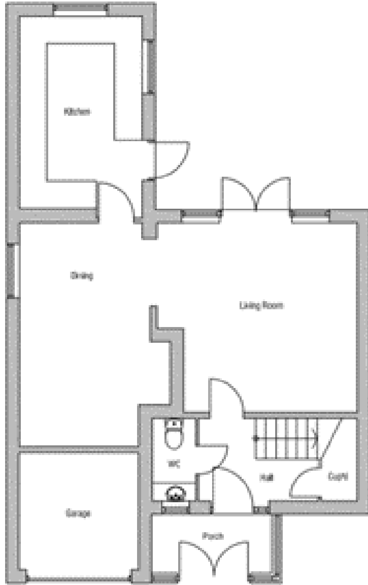
EXISTING SECOND FLOOR - 1/24
